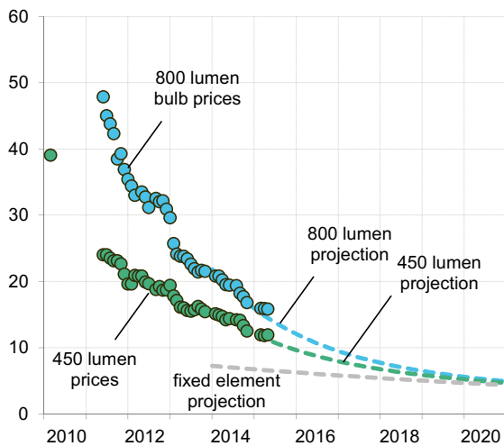
Figure 77: Global LED bulb average selling price data and projections ($)
