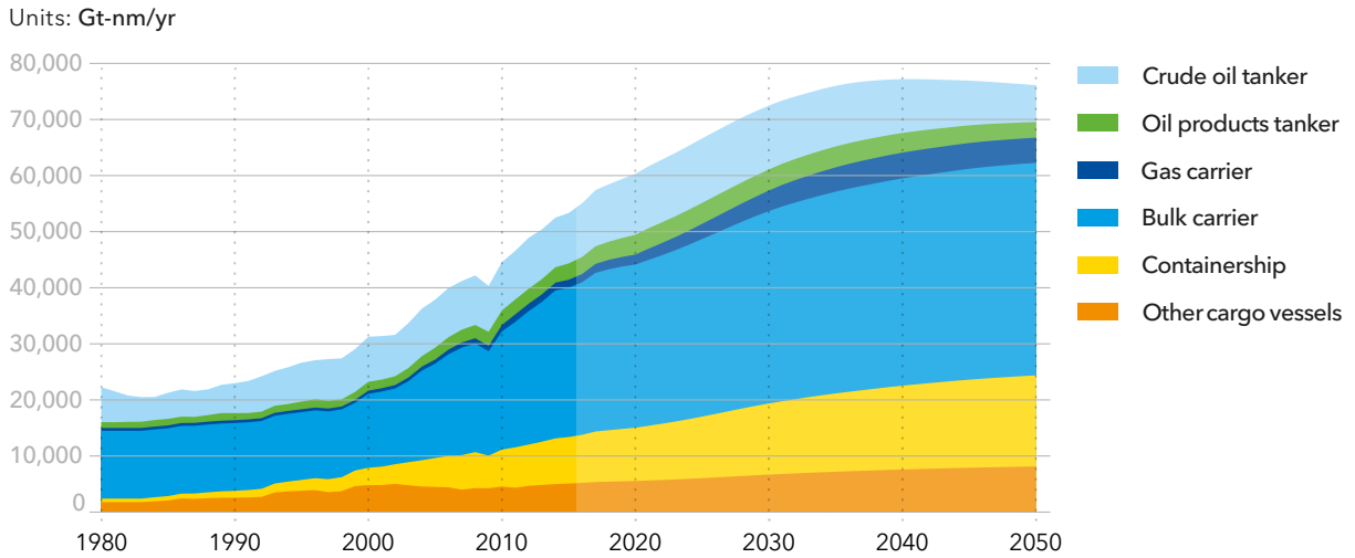
World seaborne trade in tonne-miles by vessel type
