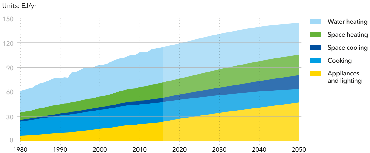
World buildings sector energy demand by end use
