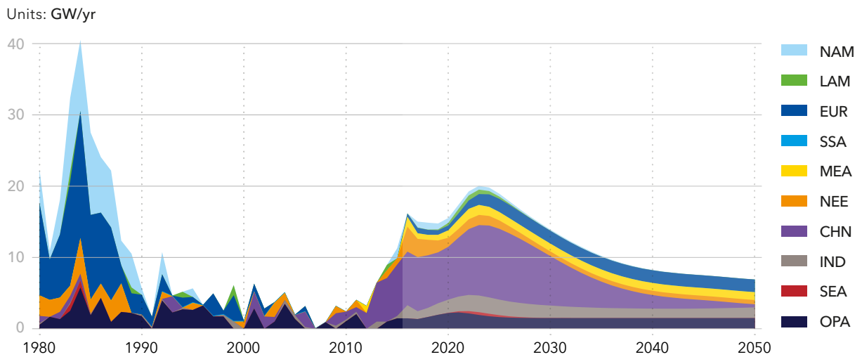
Nuclear capacity additions by region
