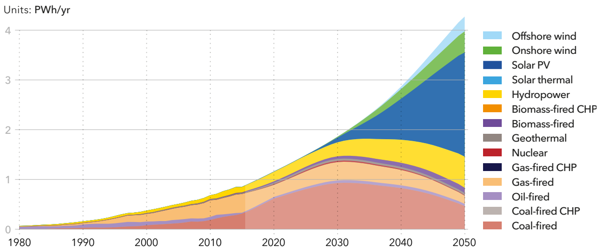
South East Asia electricity generation by power station type
