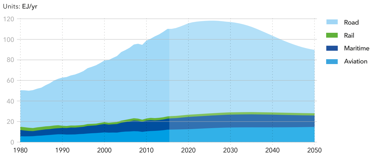
World transport sector energy demand by sub-sector
