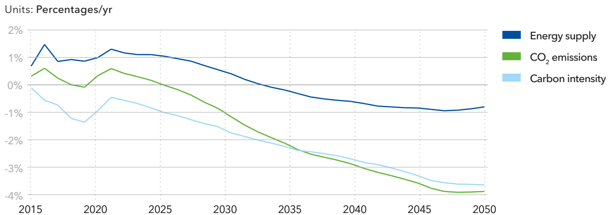
Carbon intensity, energy supply and emissions rate of change
