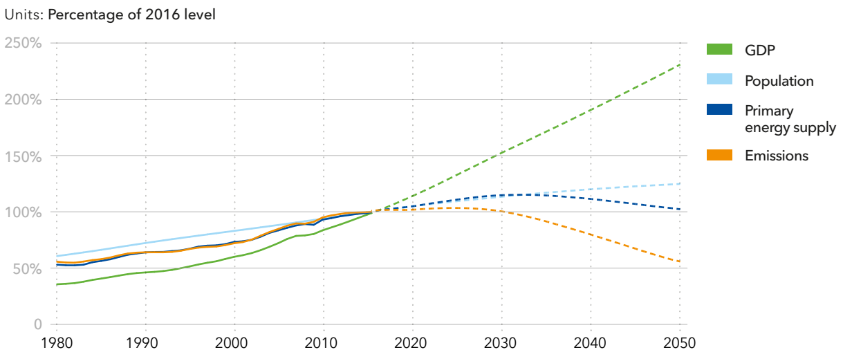
Relationship between world population, GDP, energy supply and emissions
