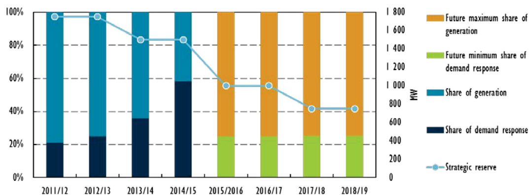
Figure 5.3 • Development of Swedish strategic reserve
