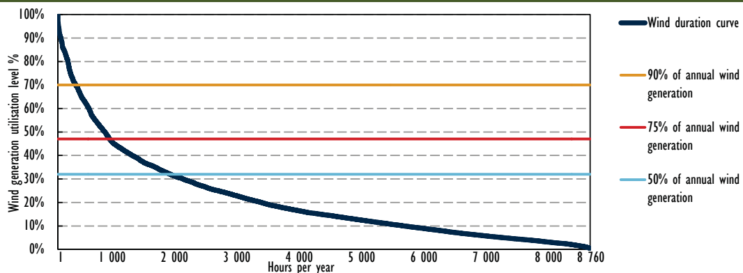
Figure 8.6 • Annual generation wind duration curve in Germany
