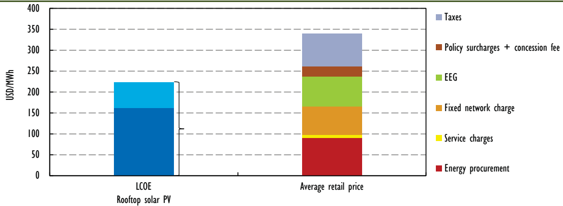
Figure 9.6 • Comparison of LCOE for PV and the average retail price in Germany
