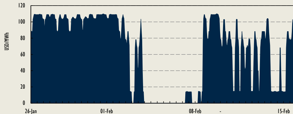
Figure 2.4 • Electricity prices, three weeks in 2050
