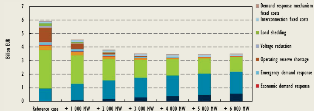
Figure 4.4 • Total reliability costs for different gas-fired capacity additions
