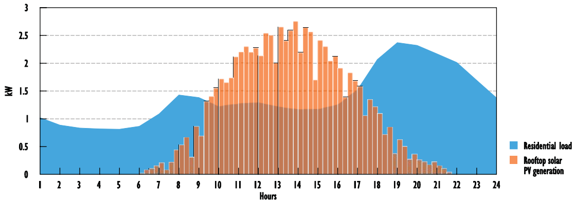
Figure 9.10 • An example of hourly profile of household load and solar PV generation (illustrative)
