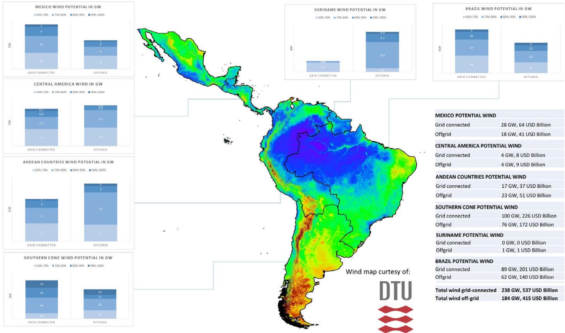
Figure 4: Wind energy - Grid-connected and utility scale off-grid technical potential estimates for Latin American by region, expressed in GW and USD. The suitability threshold is 60% and the output is indicated for a grid distance of 75 km.
